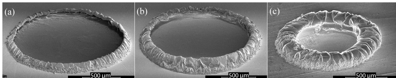
FIG. 2. SEM images of deposits with different morphologies: (a) open shell, (b) intermediate open shell, and (c) closed shell.
